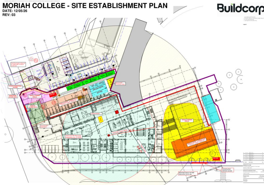
Figure 6 - Methodology (Main Works), Prepared by Buildcorp
