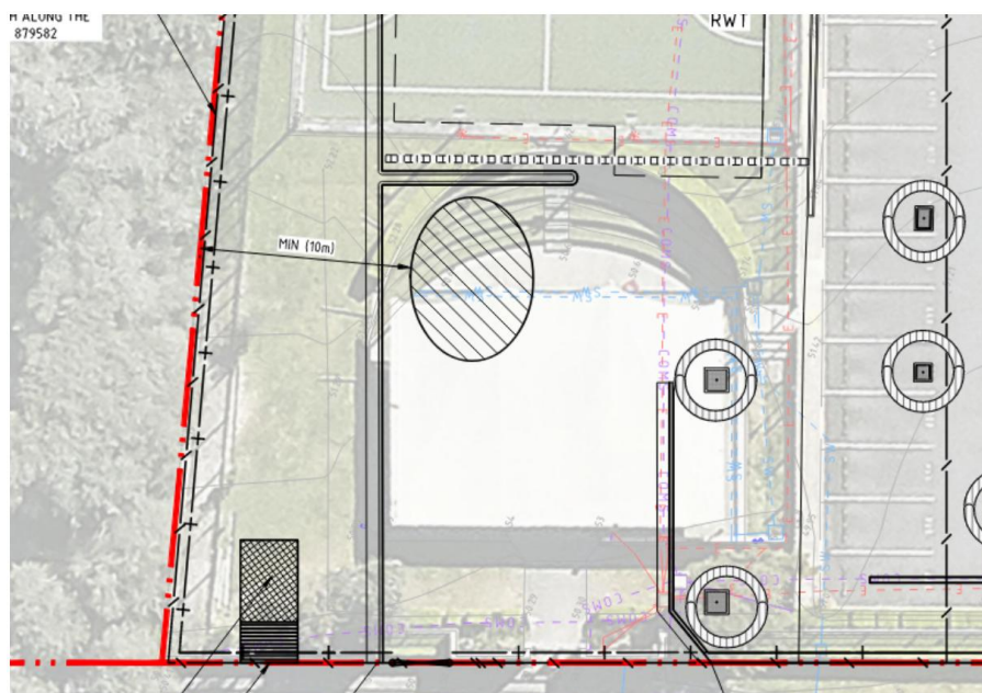
Figure 3 - Proposed Site Storage Stockpile Locations (Enabling), extract of Sediment and Soil Erosion Control Plan
