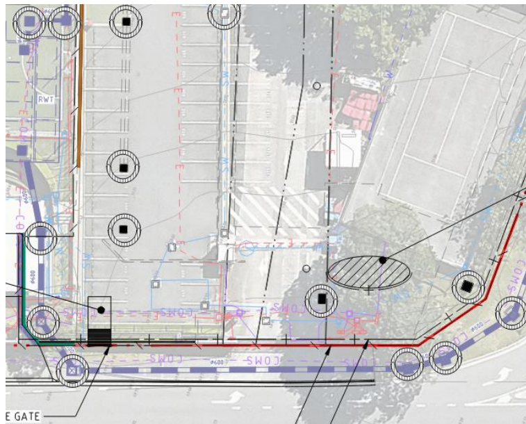
Figure 5 - Proposed Site Storage Stockpile Locations (Main), extract of Sediment and Soil Erosion Control Plan
